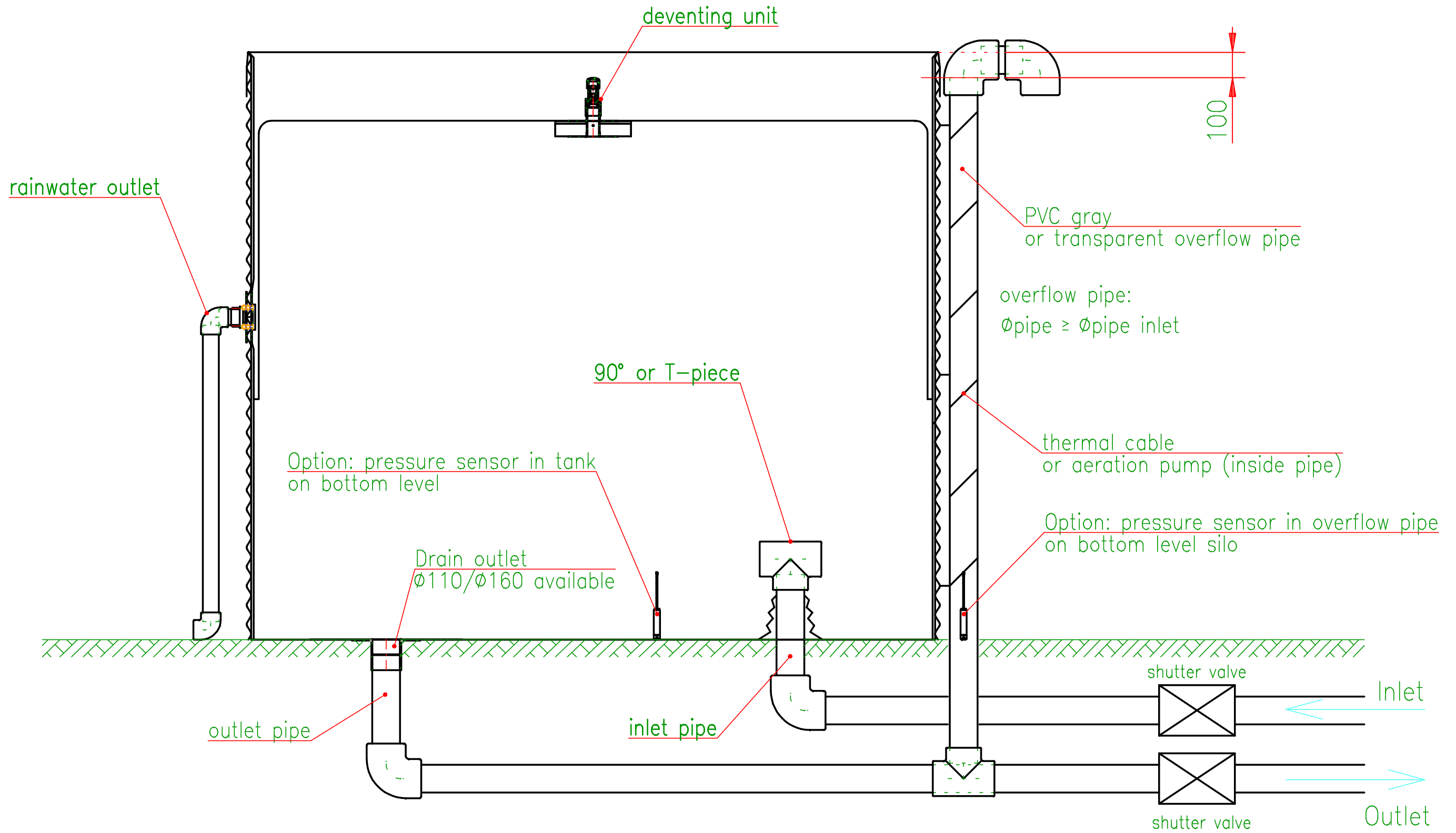
Silo cross section with GenaFlexstore
